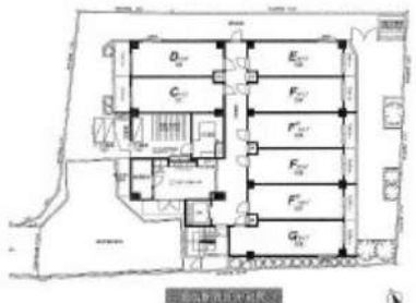
FLOOR PLAN
